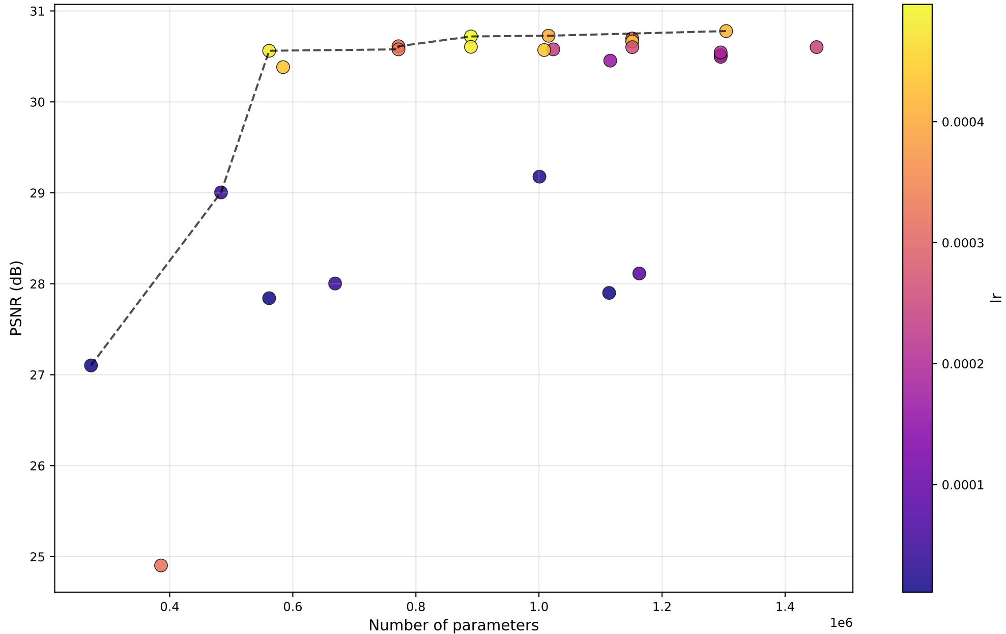
PSNR vs #Params — OmniSR — by l_r
